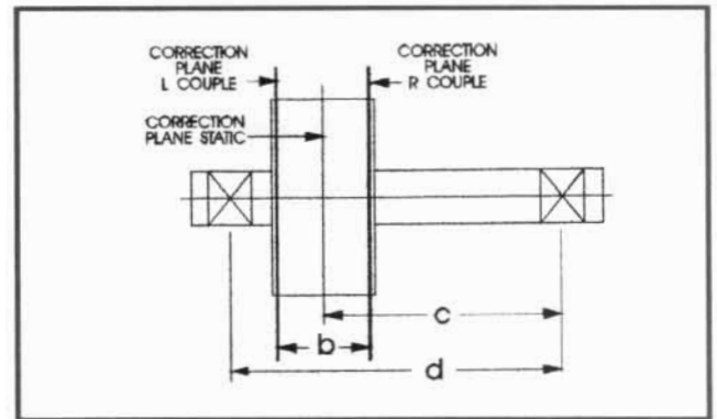
Figure 5 Narrow rotors
