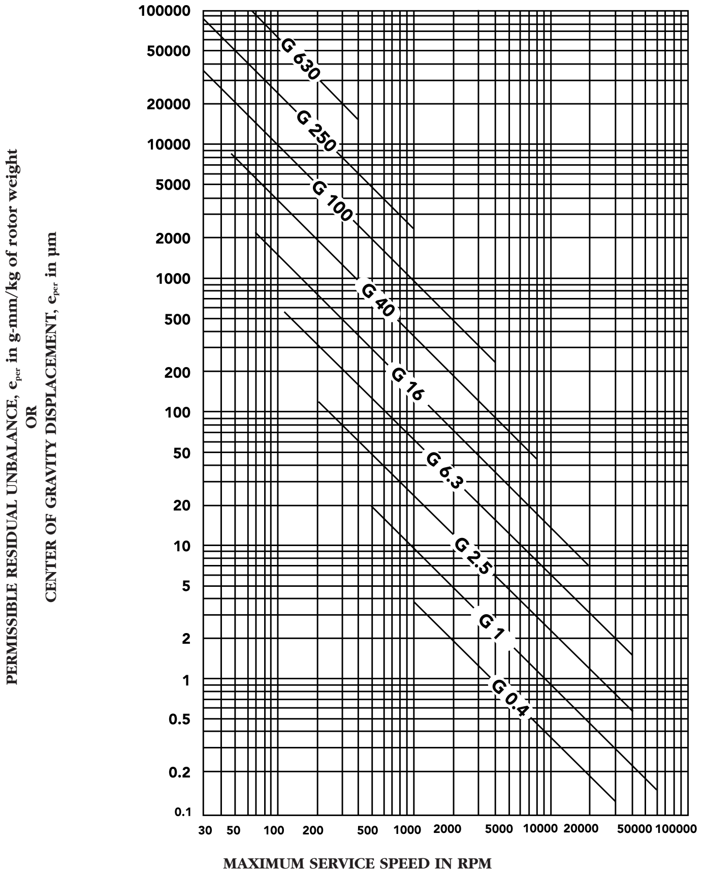
Figure 1-B Maximum permissible residual unbalance, e_{\text{per}} (From ISO 1940/1)
