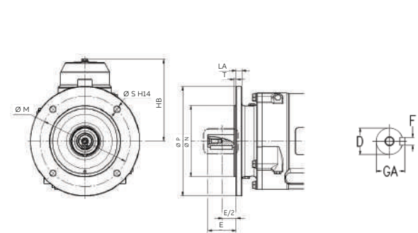
Flange-mounted B5
