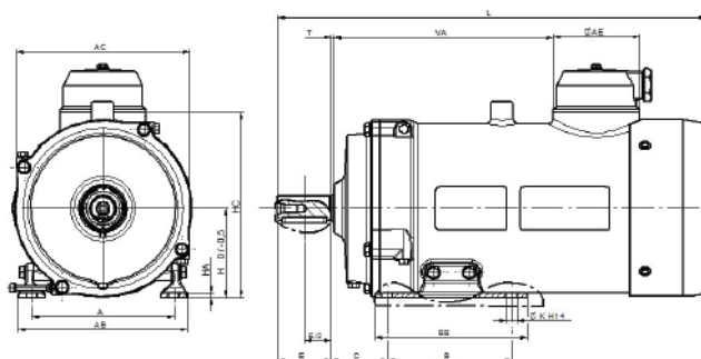
Foot-mounted B3
