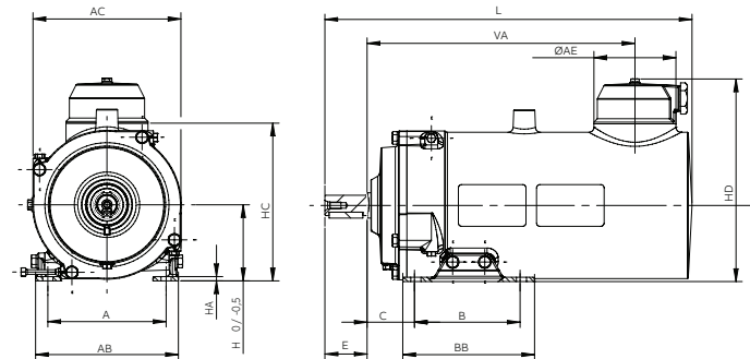
Foot-mounted B3
