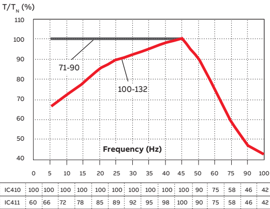
IC410 Non ventilated natural air flow, IEC frame sizes 71-90 IC410 Self ventilated, IEC frame size 100-132
