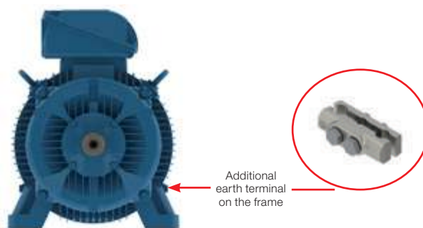
Figure 8 - Additional earth terminal position on the frame.
