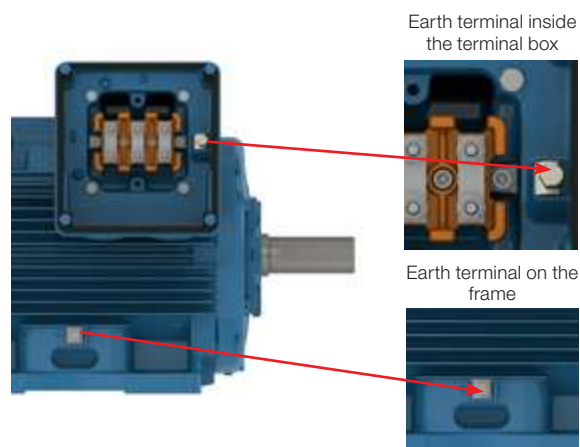
Figure 7 - Earth terminal inside the terminal box
