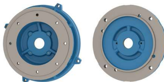
Figure 13 - C and D flanged end shields
