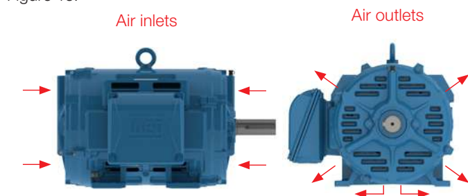
Figure 16 – Motor's air inlets and outlets.
