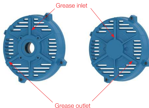
Figure 12 - Drive and non-drive end shields
